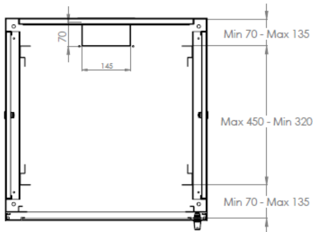
MAX/STD/MIN EQUIPMENT MOUNTING DISTANCE
