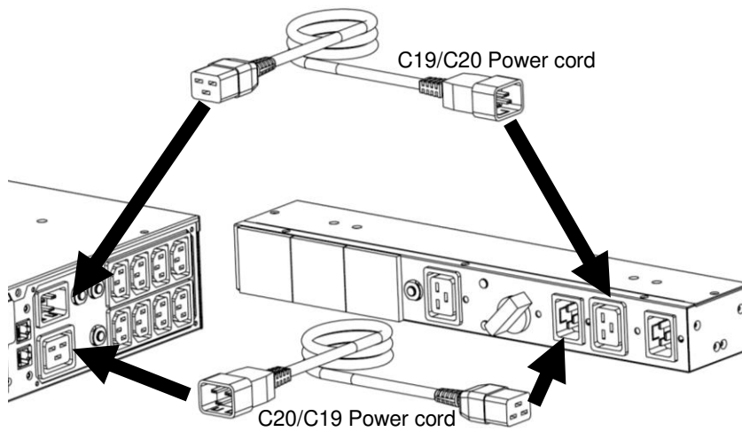
3K configuration
