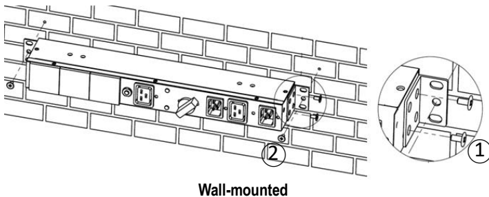
Wall-mounted
